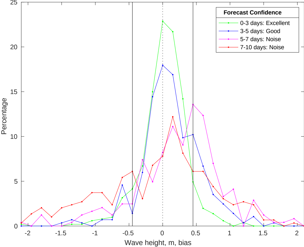
NDBC 46059 vs CMEMS Waves Bias Histogram: 13-Jan-2026
