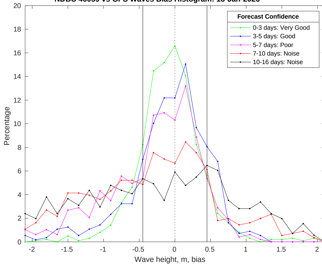
NDBC 46059 vs GFS Waves Bias Histogram: 13-Jan-2026
