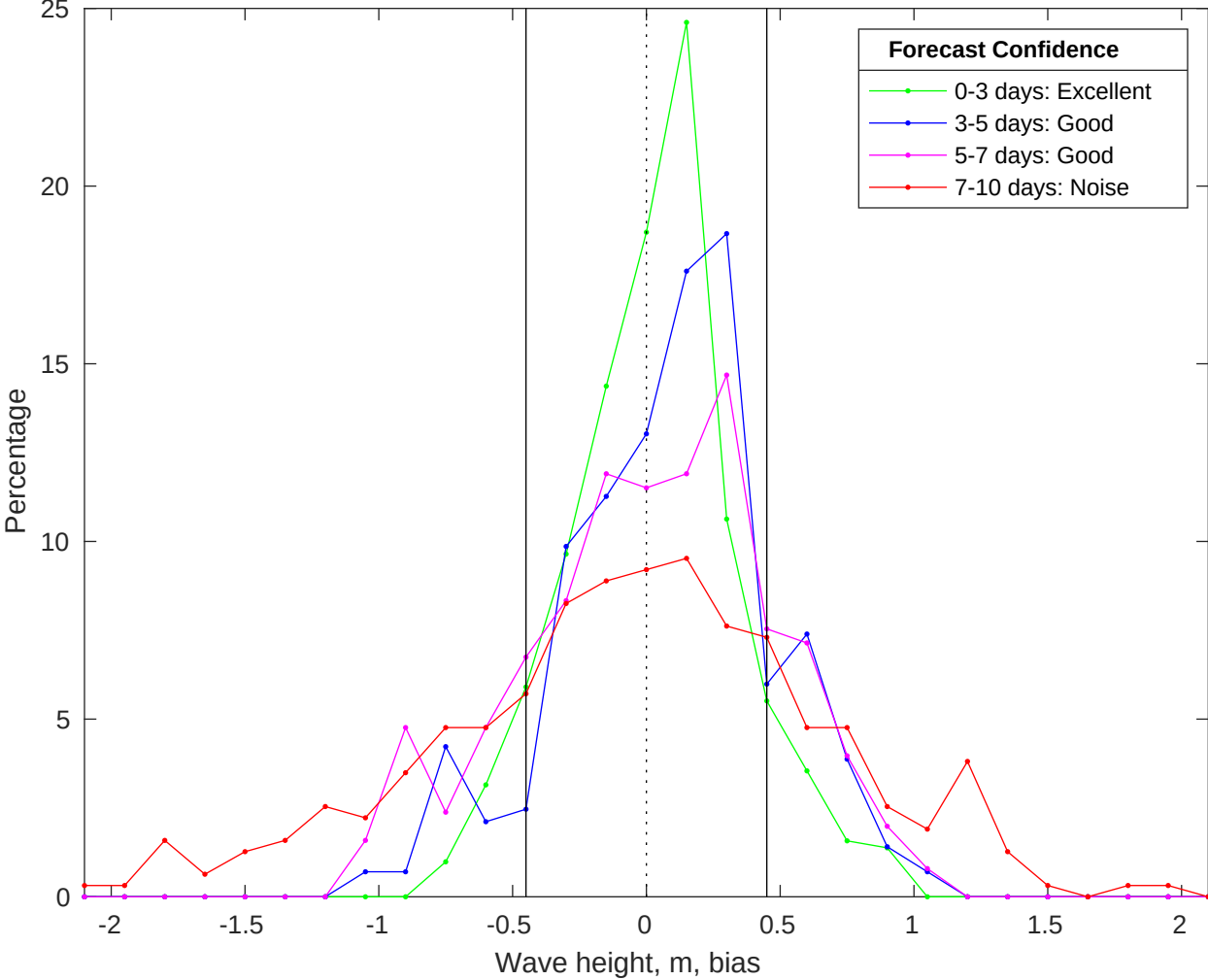
NDBC 46069 vs CMEMS Waves Bias Histogram: 13-Jan-2026
