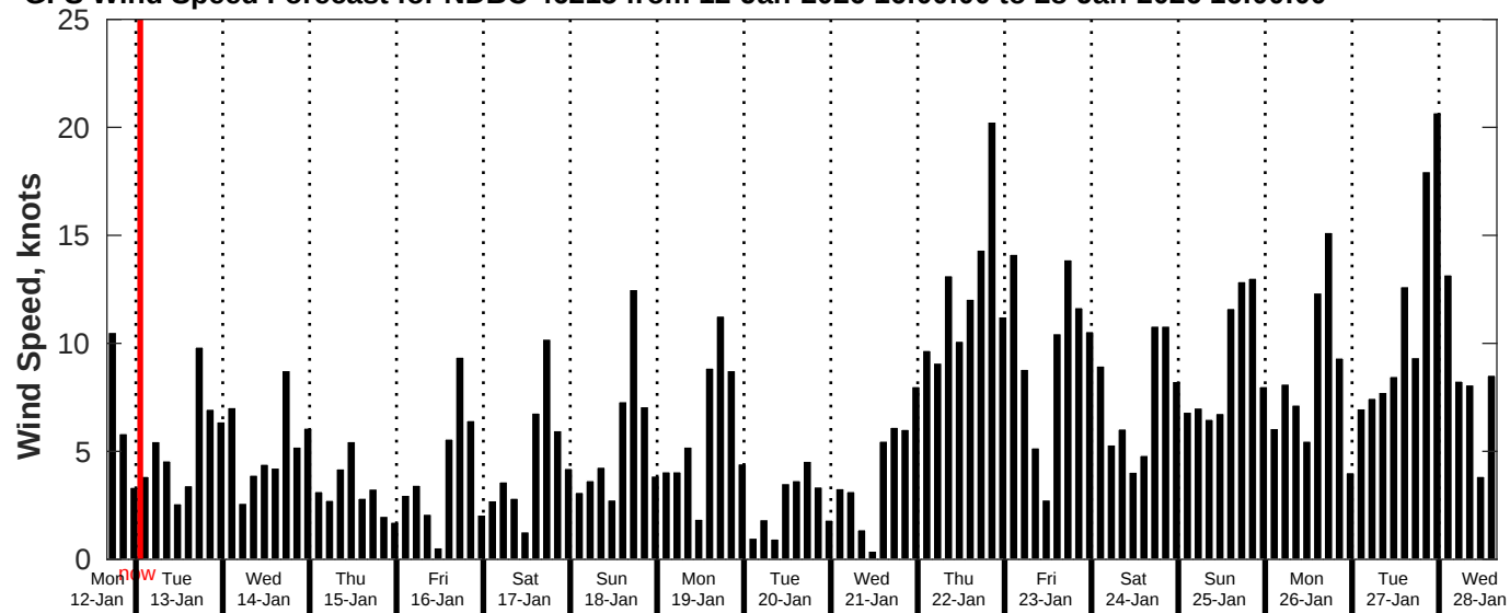
GFS Wind Speed Forecast for NDBC 46215 from 12-Jan-2026 16:00:00 to 28-Jan-2026 16:00:00
