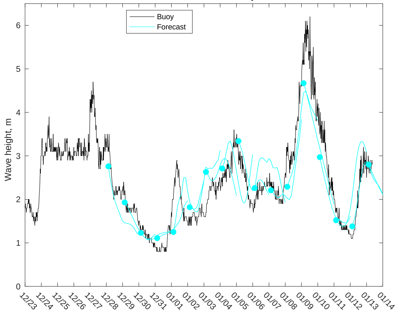
NDBC 46259 vs CMEMS Waves: 5 to 7 day forecast
