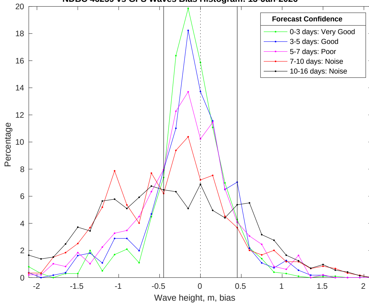
NDBC 46259 vs GFS Waves Bias Histogram: 13-Jan-2026
