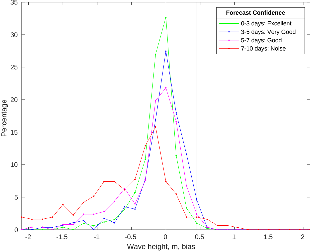
NDBC 51000 vs CMEMS Waves Bias Histogram: 13-Jan-2026
