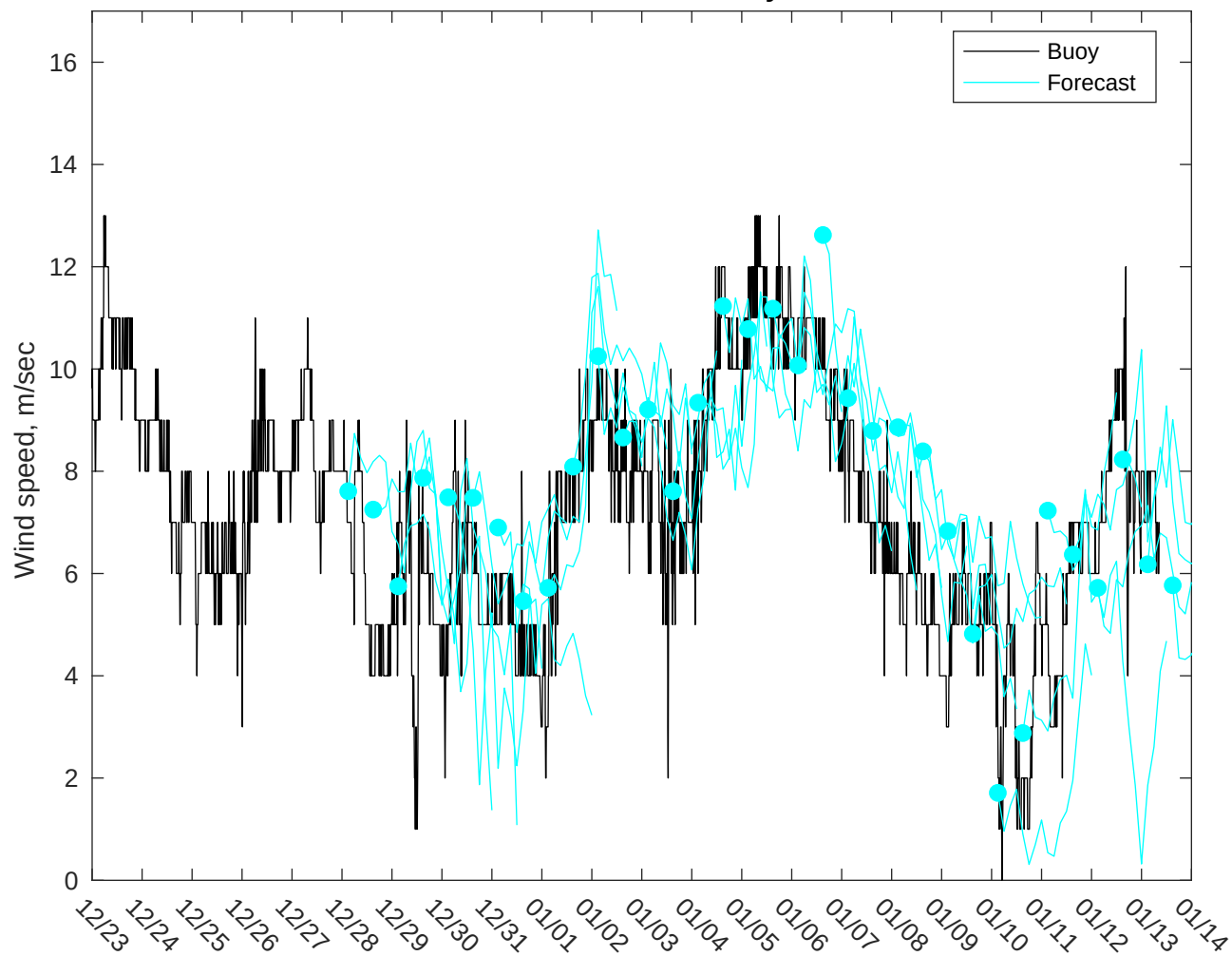
NDBC 51000 vs GFS Winds: 5 to 7 day forecast
