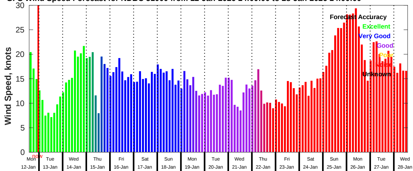
GFS Wind Speed Forecast for NDBC 51000 from 12-Jan-2026 14:00:00 to 28-Jan-2026 14:00:00
