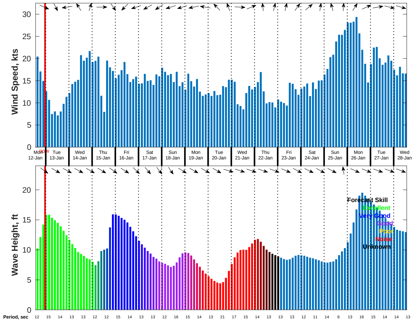
Wind & Wave Forecast for NDBC 51000 from 12-Jan-2026 14:00:00 to 28-Jan-2026 14:00:00
