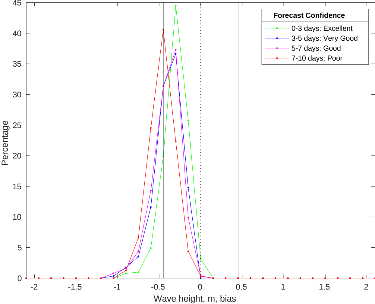
NDBC 51209 vs CMEMS Waves Bias Histogram: 13-Jan-2026
