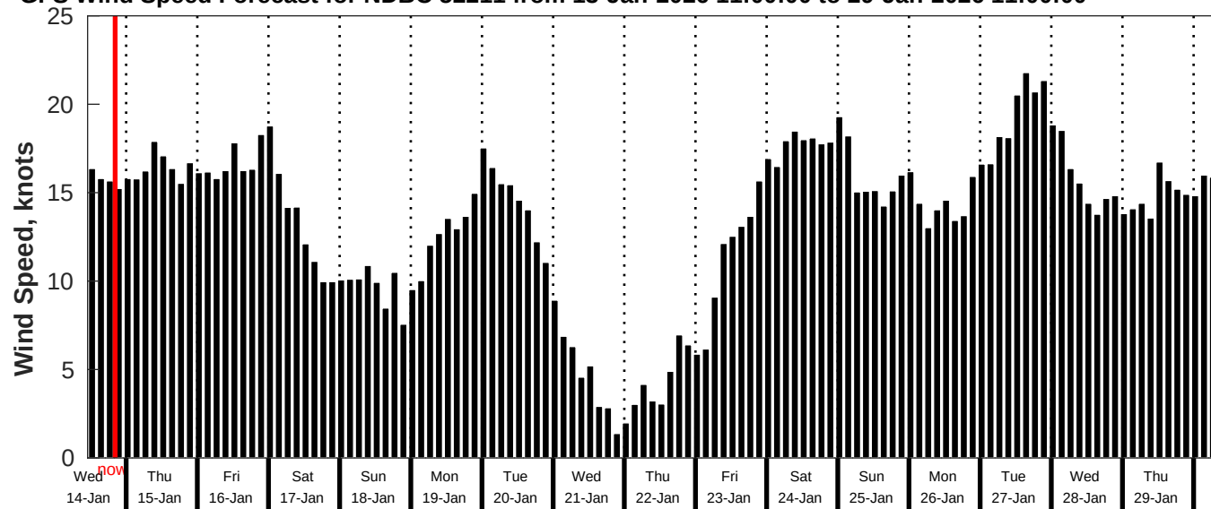
GFS Wind Speed Forecast for NDBC 52211 from 13-Jan-2026 11:00:00 to 29-Jan-2026 11:00:00
