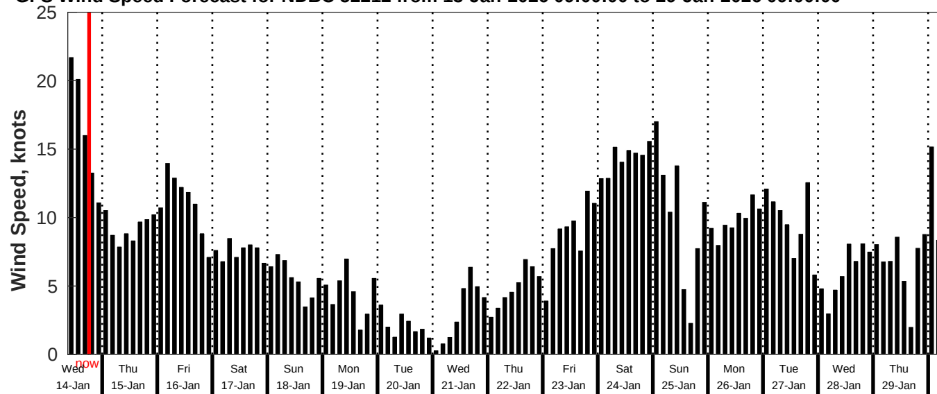
GFS Wind Speed Forecast for NDBC 52212 from 13-Jan-2026 09:00:00 to 29-Jan-2026 09:00:00
