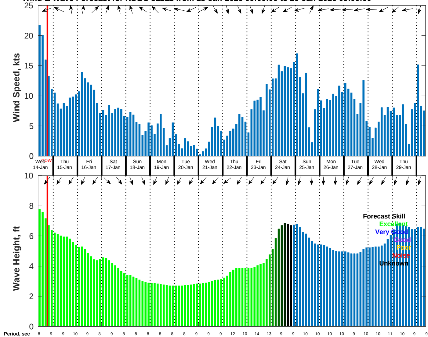
Wind & Wave Forecast for NDBC 52212 from 13-Jan-2026 09:00:00 to 29-Jan-2026 09:00:00
