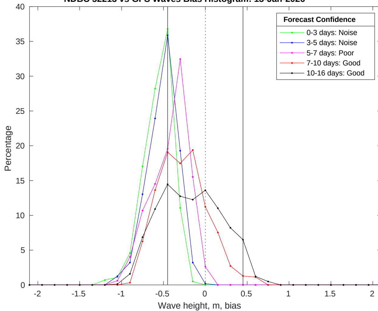
NDBC 52213 vs GFS Waves Bias Histogram: 13-Jan-2026
