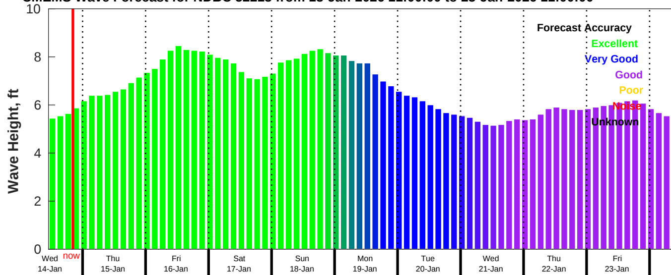
CMEMS Wave Forecast for NDBC 52213 from 13-Jan-2026 11:00:00 to 23-Jan-2026 11:00:00
