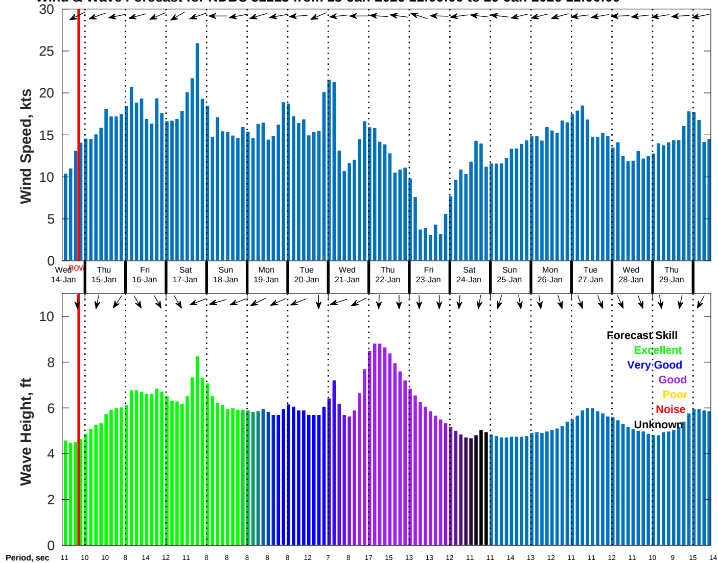
Wind & Wave Forecast for NDBC 52213 from 13-Jan-2026 11:00:00 to 29-Jan-2026 11:00:00
