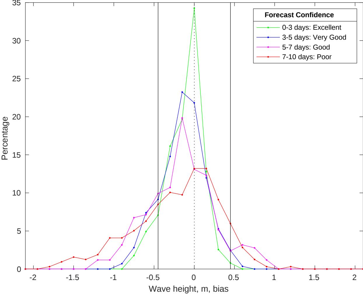
NDBC 41004 vs CMEMS Waves Bias Histogram: 14-Jan-2026
