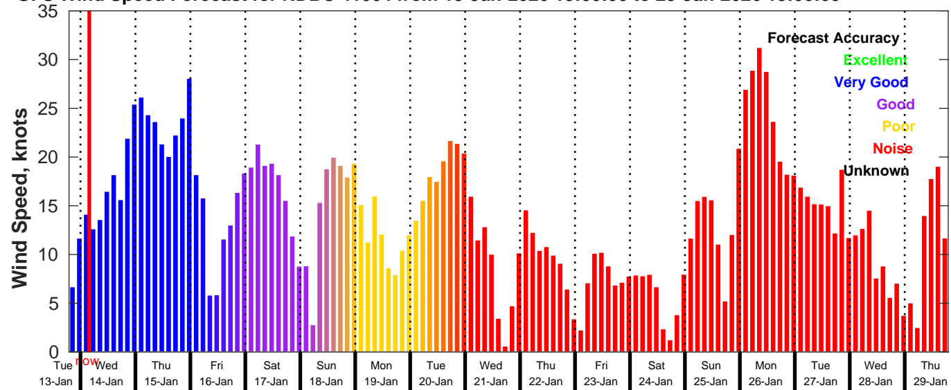
GFS Wind Speed Forecast for NDBC 41004 from 13-Jan-2026 19:00:00 to 29-Jan-2026 19:00:00
