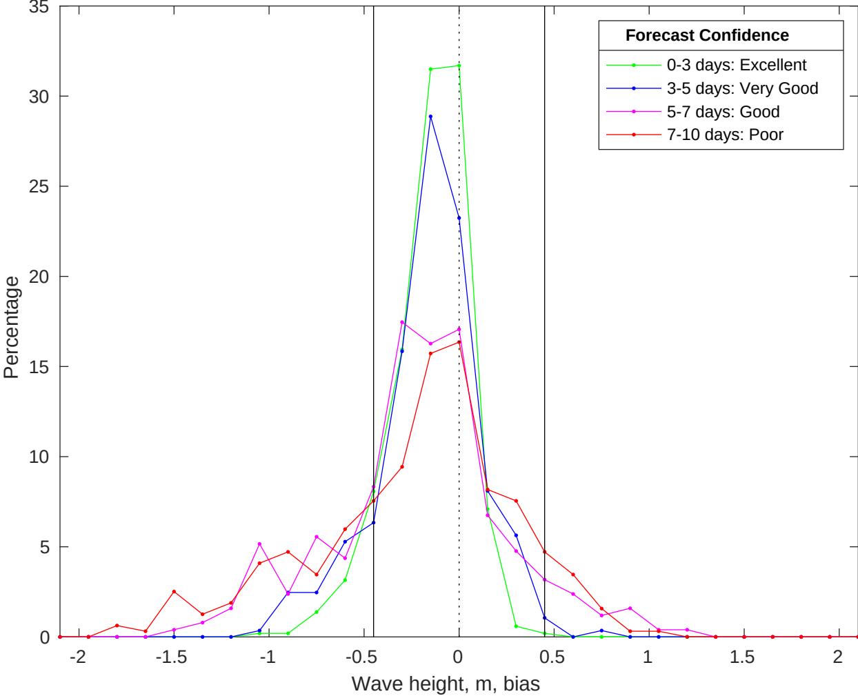
NDBC 41013 vs CMEMS Waves Bias Histogram: 14-Jan-2026
