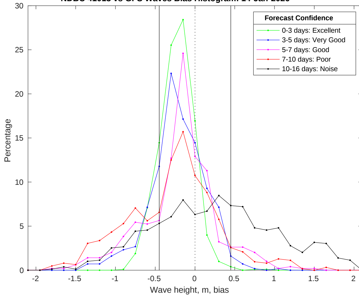
NDBC 41013 vs GFS Waves Bias Histogram: 14-Jan-2026
