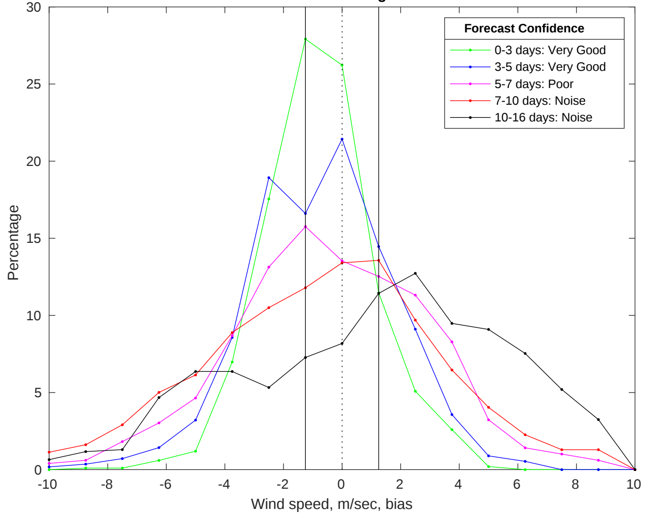
NDBC 41013 vs GFS Winds Bias Histogram: 14-Jan-2026
