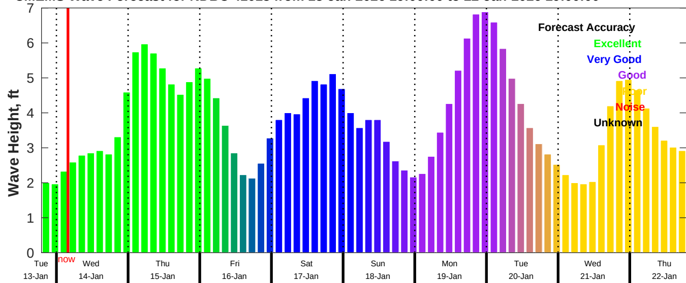
CMEMS Wave Forecast for NDBC 41013 from 13-Jan-2026 19:00:00 to 22-Jan-2026 19:00:00
