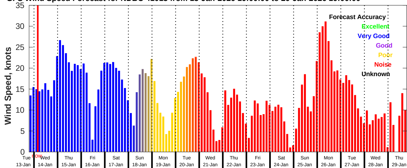
GFS Wind Speed Forecast for NDBC 41013 from 13-Jan-2026 19:00:00 to 29-Jan-2026 19:00:00
