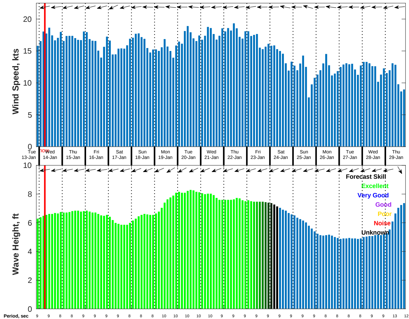
Wind & Wave Forecast for NDBC 41040 from 13-Jan-2026 21:00:00 to 29-Jan-2026 21:00:00
