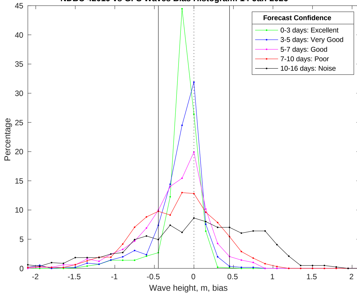
NDBC 42019 vs GFS Waves Bias Histogram: 14-Jan-2026
