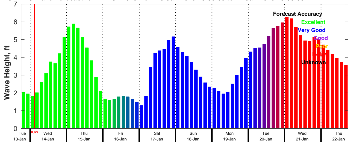
CMEMS Wave Forecast for NDBC 42019 from 13-Jan-2026 18:00:00 to 22-Jan-2026 18:00:00
