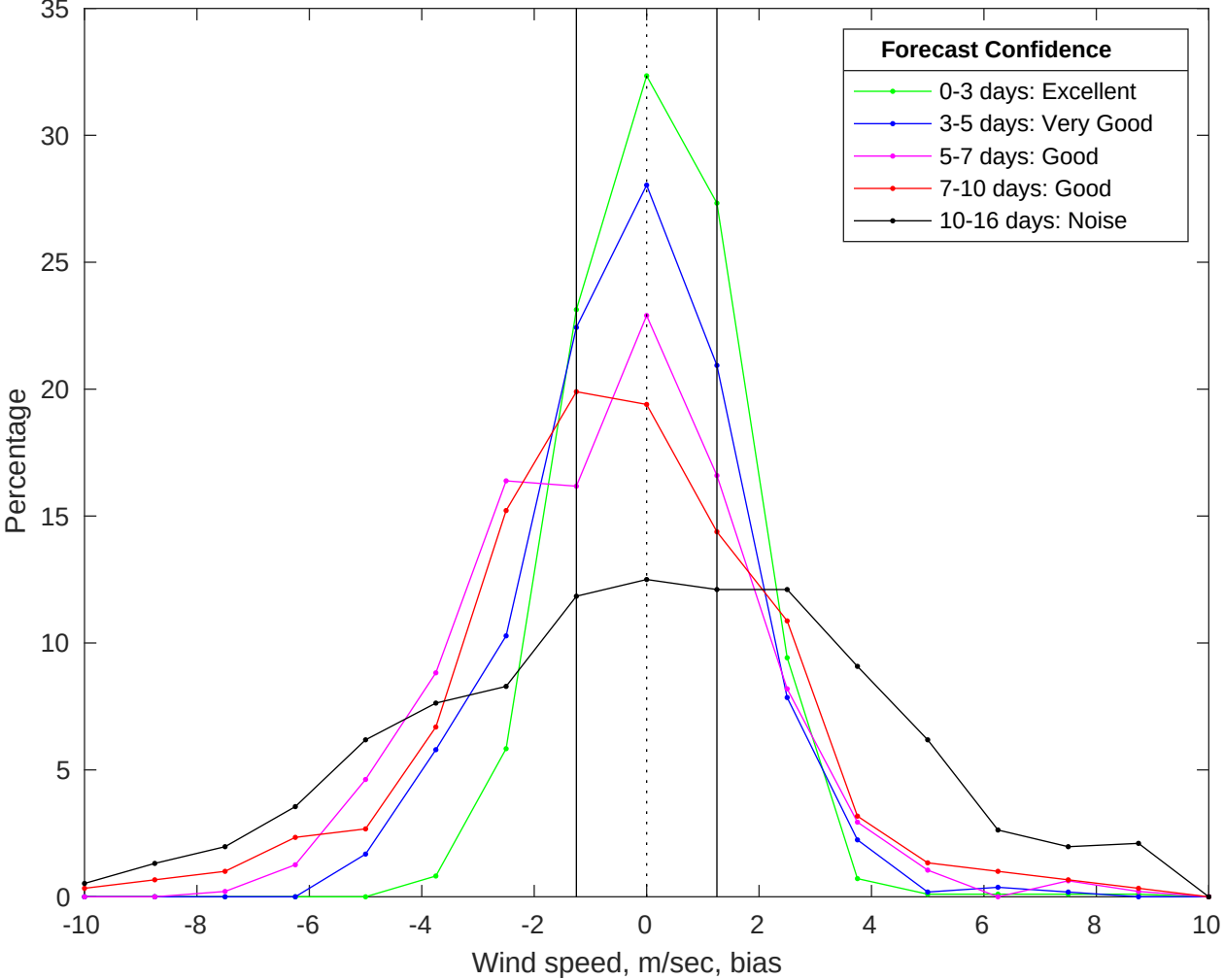
NDBC 42020 vs GFS Winds Bias Histogram: 12-Jan-2026
