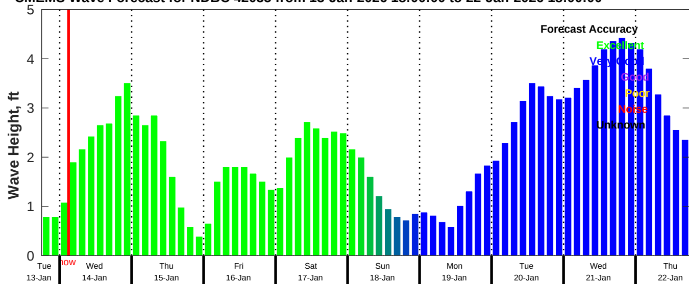
CMEMS Wave Forecast for NDBC 42035 from 13-Jan-2026 18:00:00 to 22-Jan-2026 18:00:00
