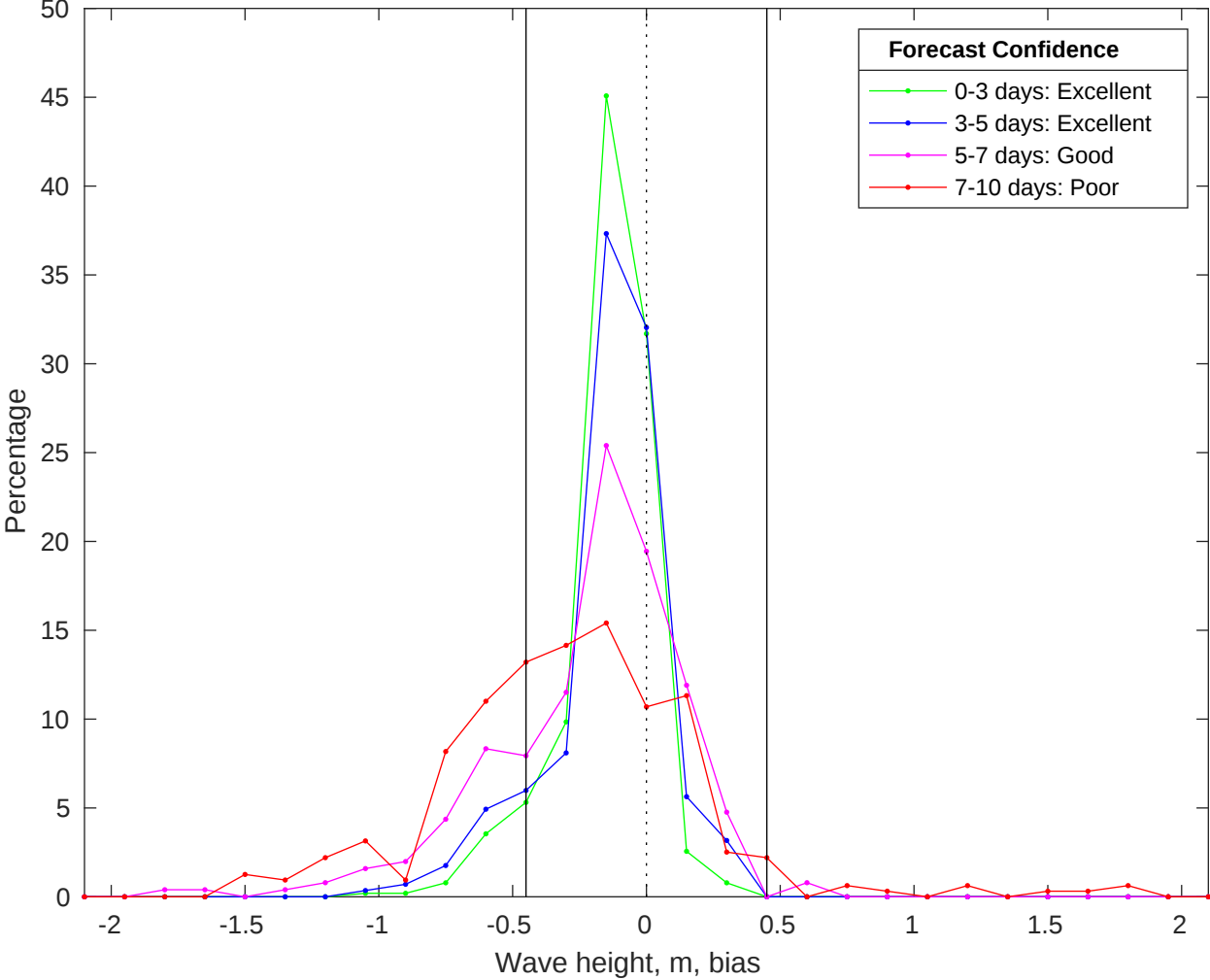
NDBC 42036 vs CMEMS Waves Bias Histogram: 14-Jan-2026
