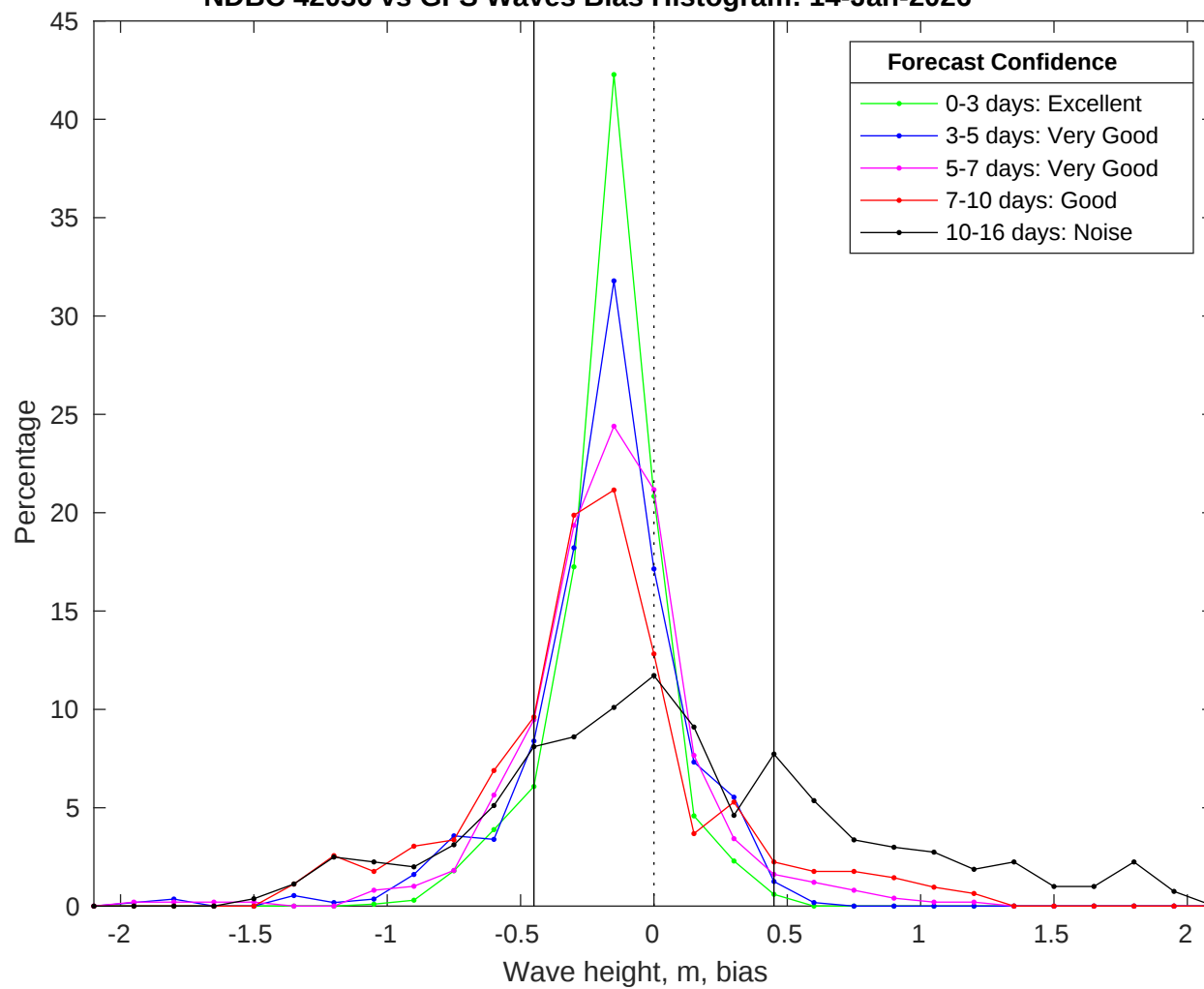
NDBC 42036 vs GFS Waves Bias Histogram: 14-Jan-2026
