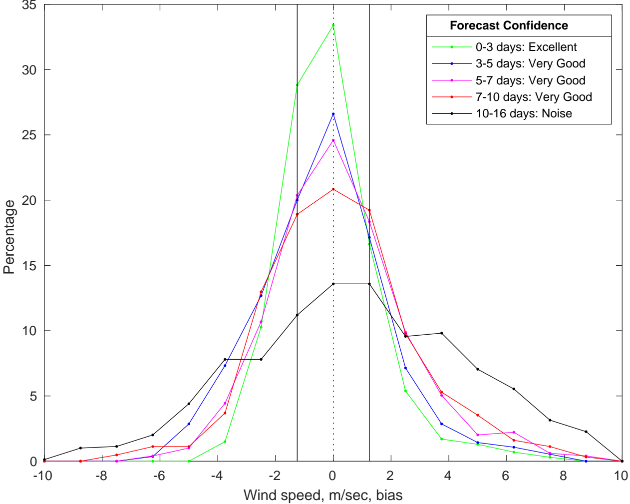
NDBC 42036 vs GFS Winds Bias Histogram: 14-Jan-2026
