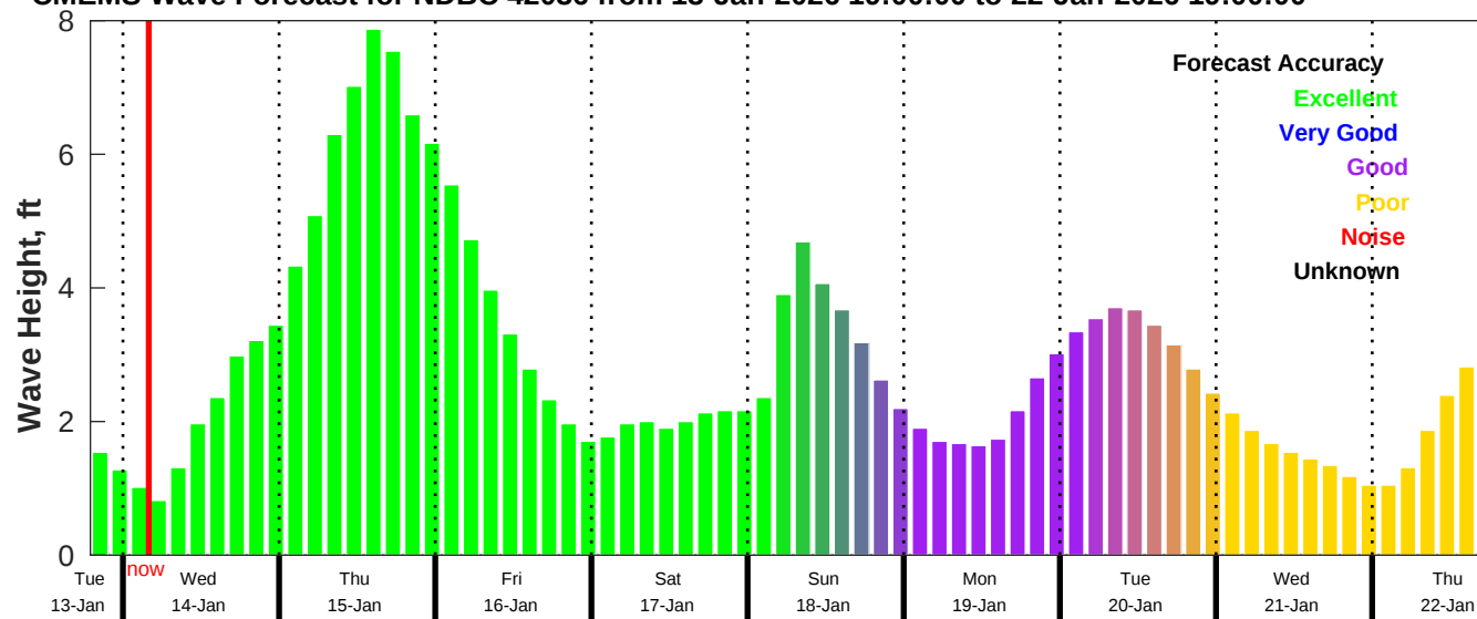
CMEMS Wave Forecast for NDBC 42036 from 13-Jan-2026 19:00:00 to 22-Jan-2026 19:00:00
