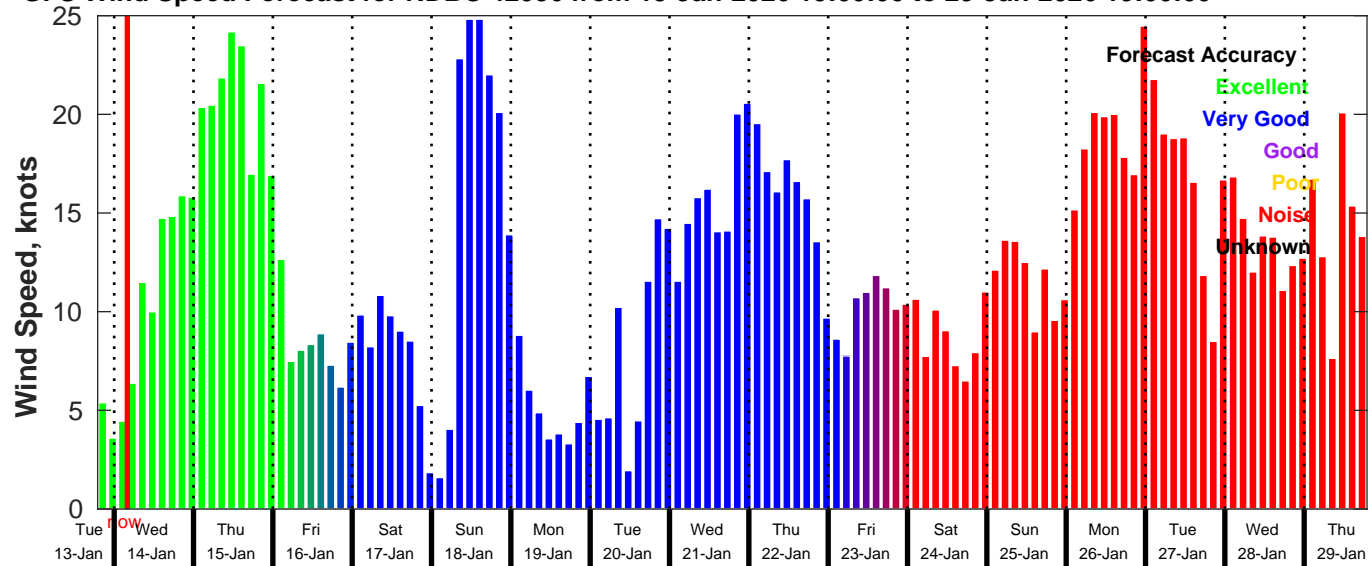
GFS Wind Speed Forecast for NDBC 42036 from 13-Jan-2026 19:00:00 to 29-Jan-2026 19:00:00
