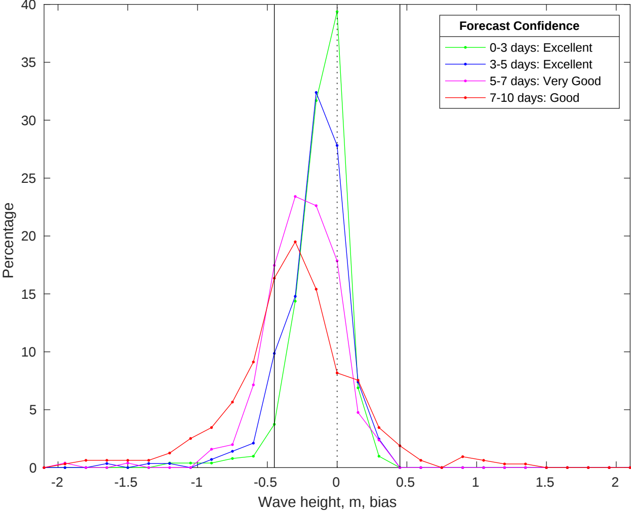
NDBC 42040 vs CMEMS Waves Bias Histogram: 14-Jan-2026
