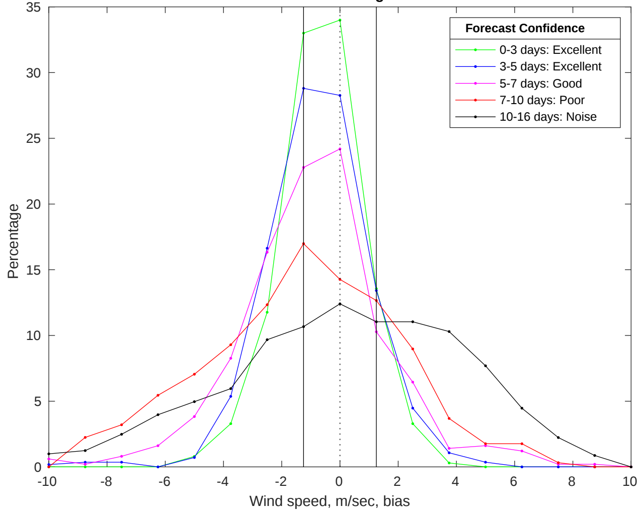
NDBC 42040 vs GFS Winds Bias Histogram: 14-Jan-2026
