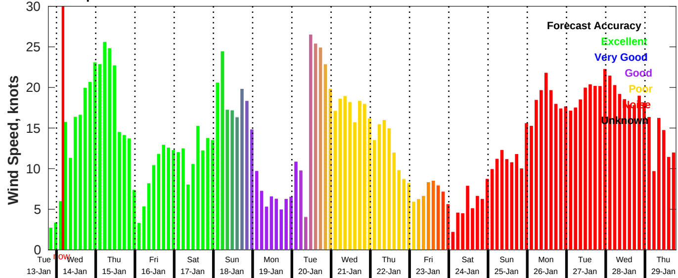
GFS Wind Speed Forecast for NDBC 42040 from 13-Jan-2026 19:00:00 to 29-Jan-2026 19:00:00
