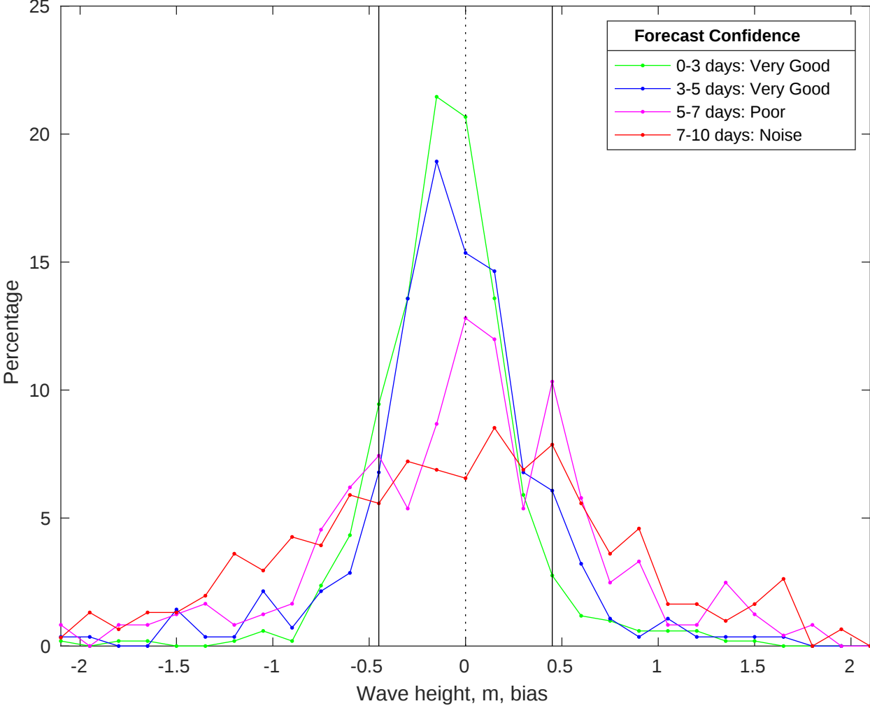
NDBC 44008 vs CMEMS Waves Bias Histogram: 14-Jan-2026
