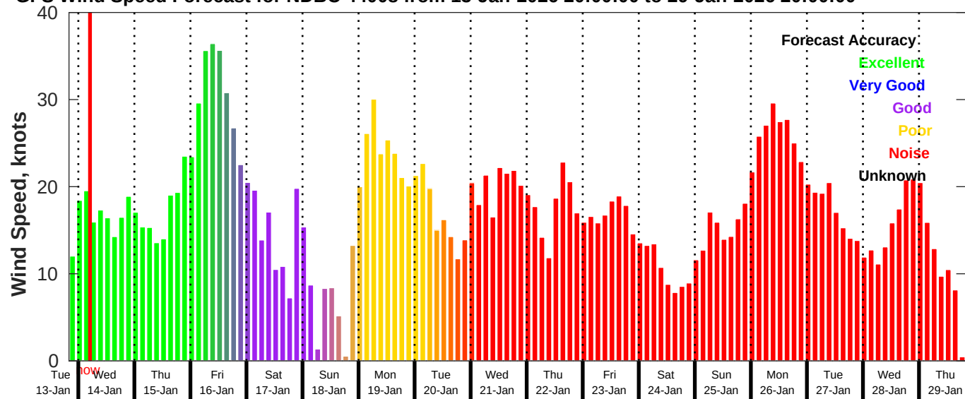
GFS Wind Speed Forecast for NDBC 44008 from 13-Jan-2026 20:00:00 to 29-Jan-2026 20:00:00
