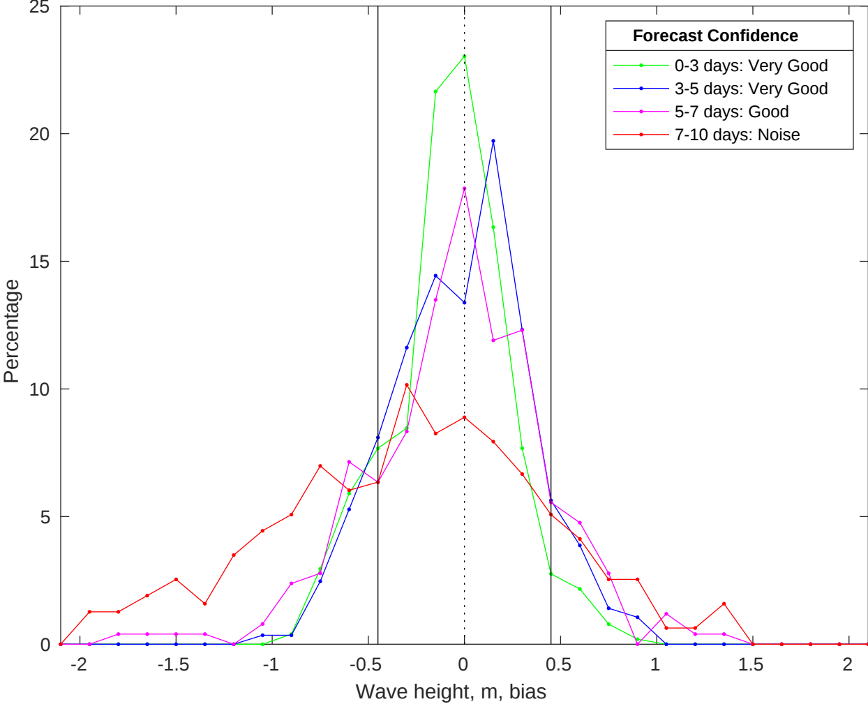
NDBC 46011 vs CMEMS Waves Bias Histogram: 14-Jan-2026
