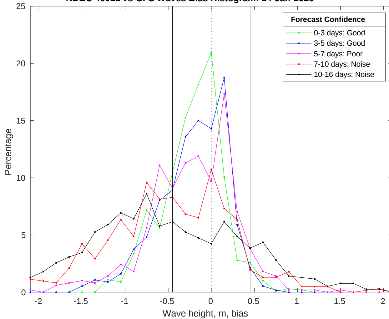
NDBC 46011 vs GFS Waves Bias Histogram: 14-Jan-2026
