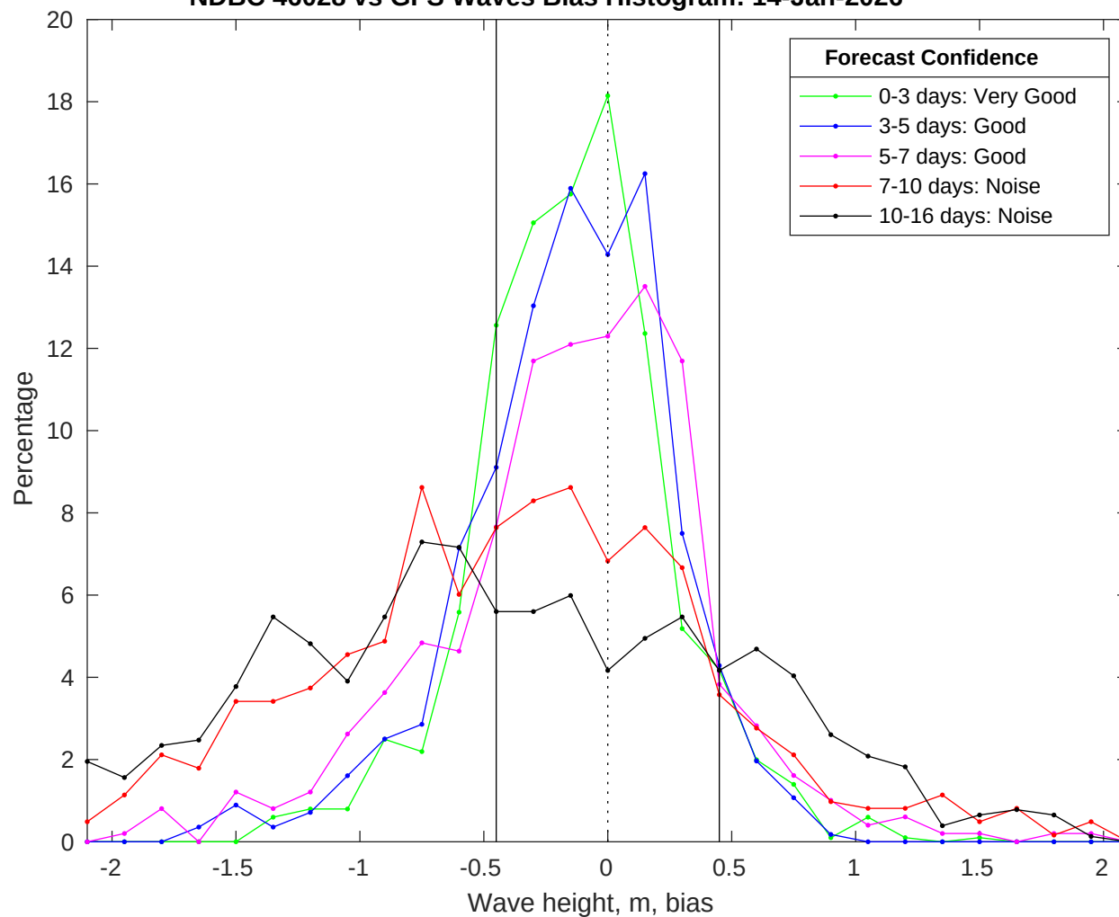
NDBC 46028 vs GFS Waves Bias Histogram: 14-Jan-2026
