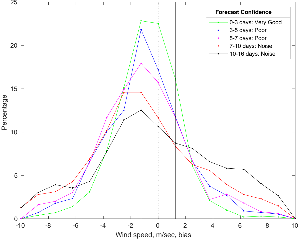
NDBC 46028 vs GFS Winds Bias Histogram: 14-Jan-2026
