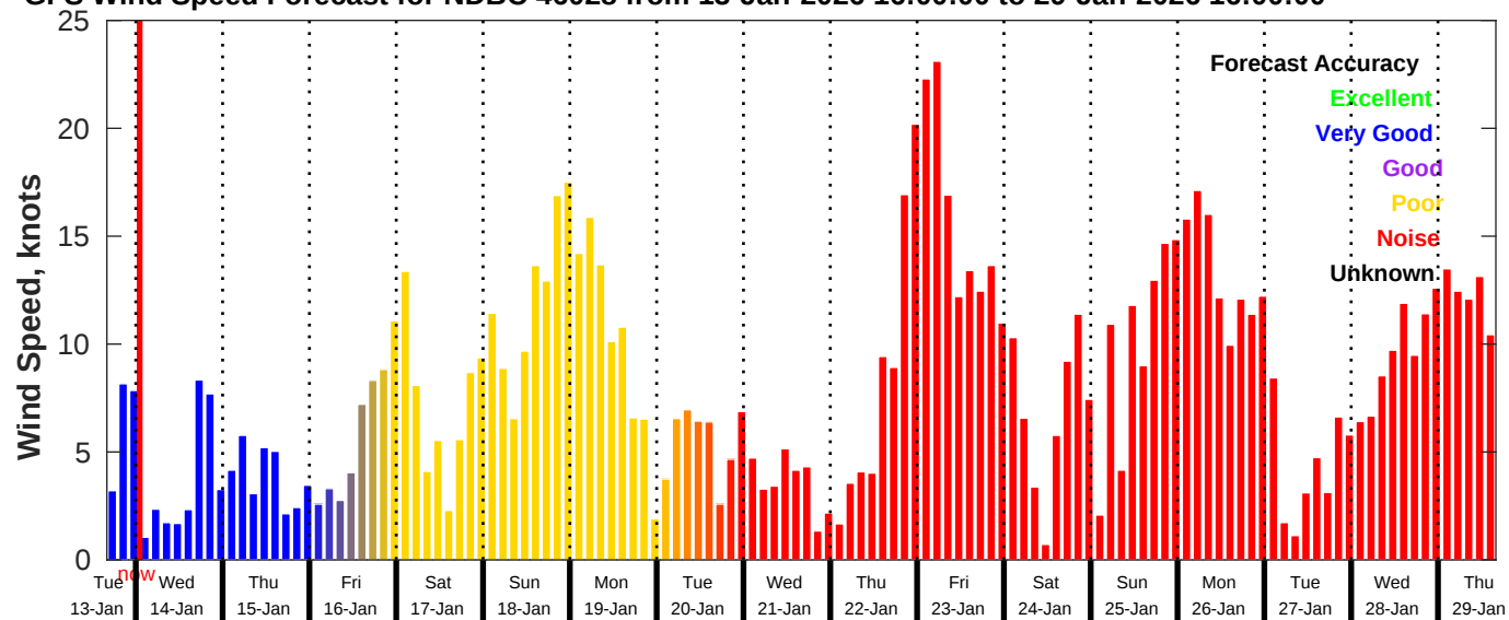
GFS Wind Speed Forecast for NDBC 46028 from 13-Jan-2026 16:00:00 to 29-Jan-2026 16:00:00
