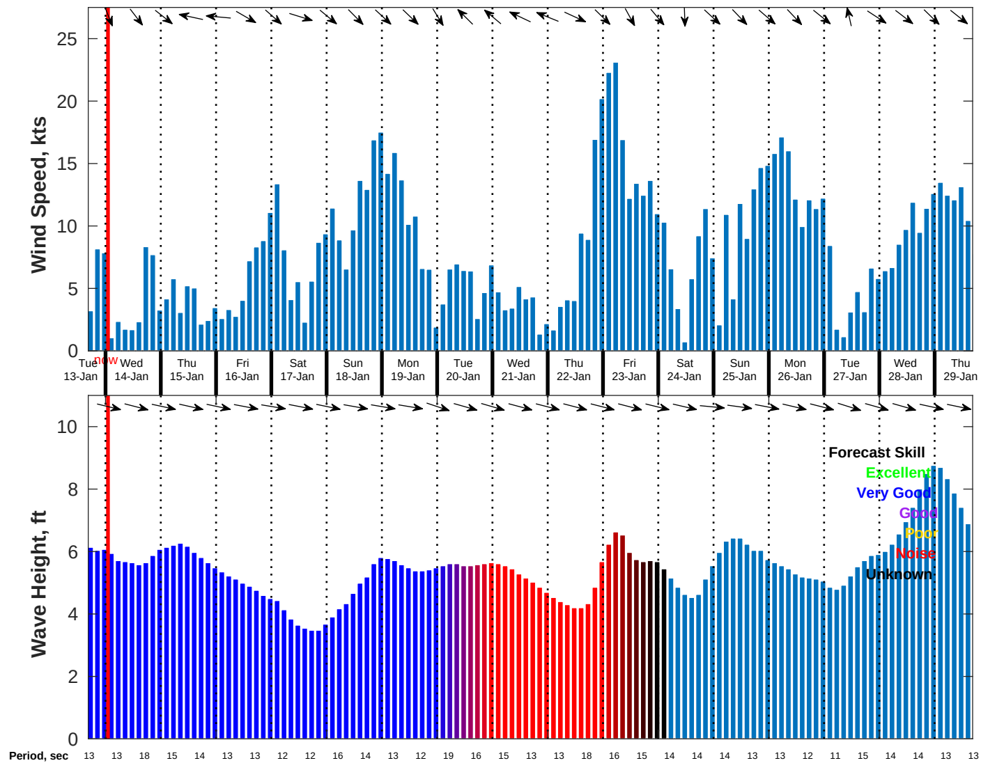
Wind & Wave Forecast for NDBC 46028 from 13-Jan-2026 16:00:00 to 29-Jan-2026 16:00:00
