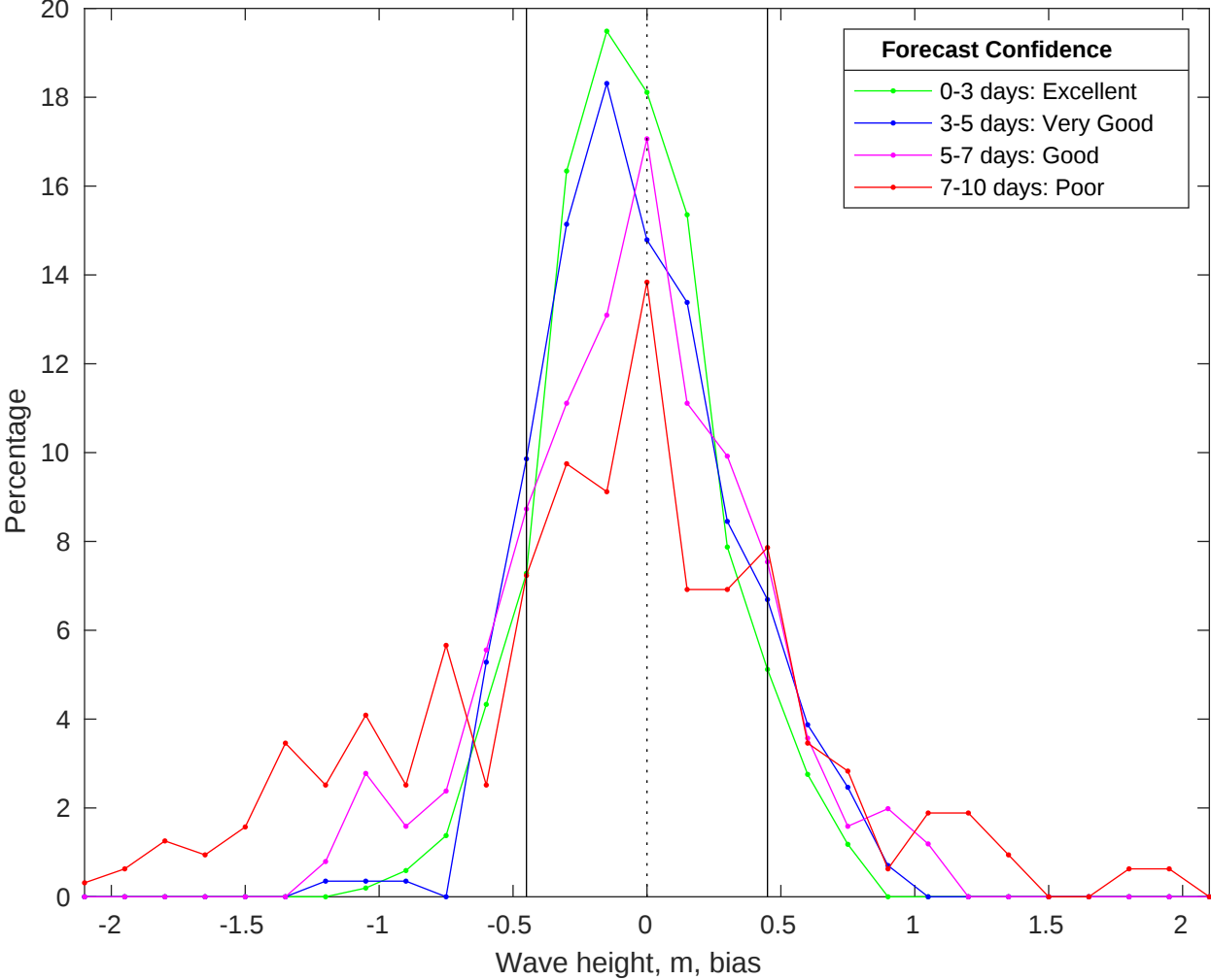
NDBC 46054 vs CMEMS Waves Bias Histogram: 14-Jan-2026
