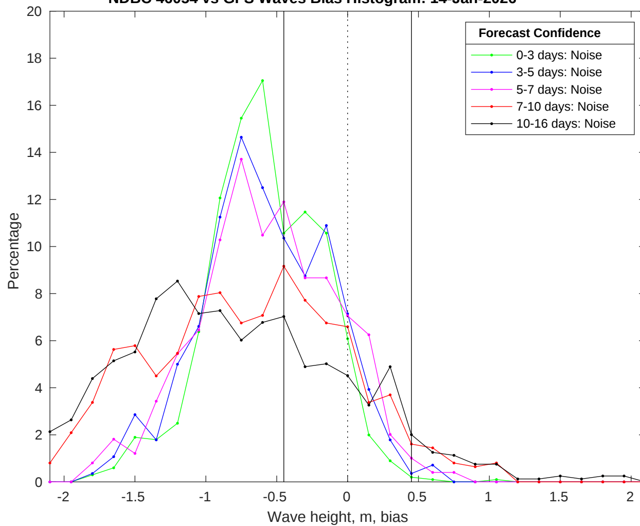
NDBC 46054 vs GFS Waves Bias Histogram: 14-Jan-2026
