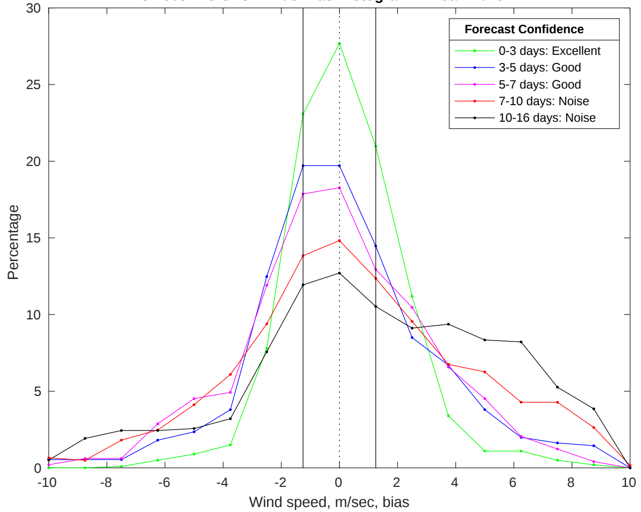
NDBC 46054 vs GFS Winds Bias Histogram: 14-Jan-2026
