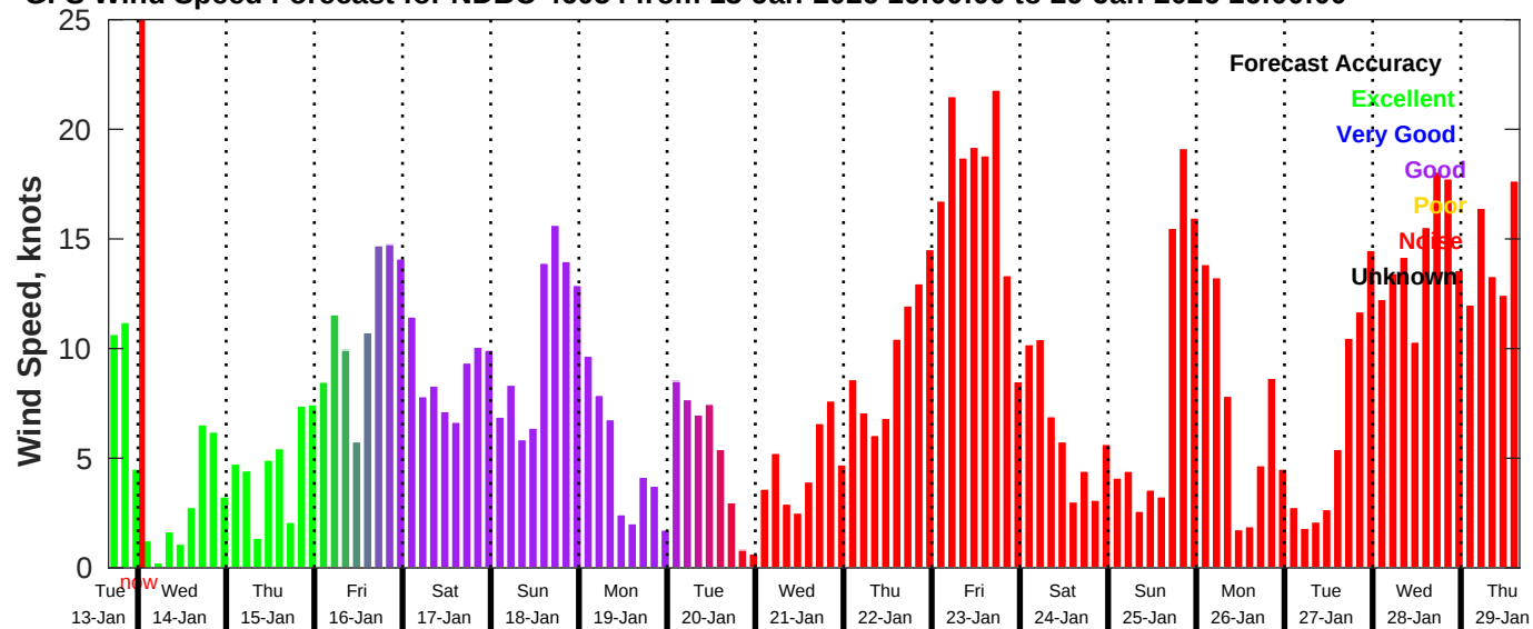
GFS Wind Speed Forecast for NDBC 46054 from 13-Jan-2026 16:00:00 to 29-Jan-2026 16:00:00
