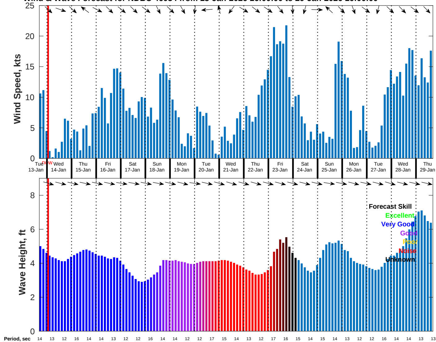
Wind & Wave Forecast for NDBC 46054 from 13-Jan-2026 16:00:00 to 29-Jan-2026 16:00:00
